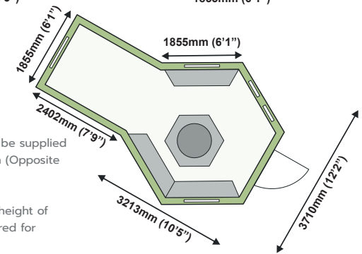
Medium Stuga floor plan extension
