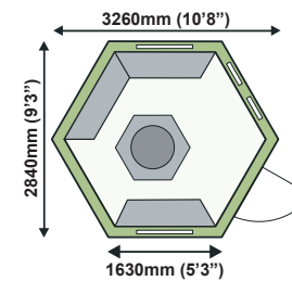
Small Stuga floor plan
