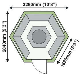
Medium garden lodge floor plan extension:
