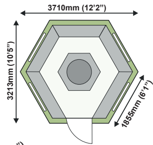
Medium garden lodge floor plan: (seating capacity - 15+)
